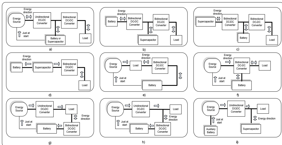
Fig. 1. Different all-EV configurations reported in literature.
