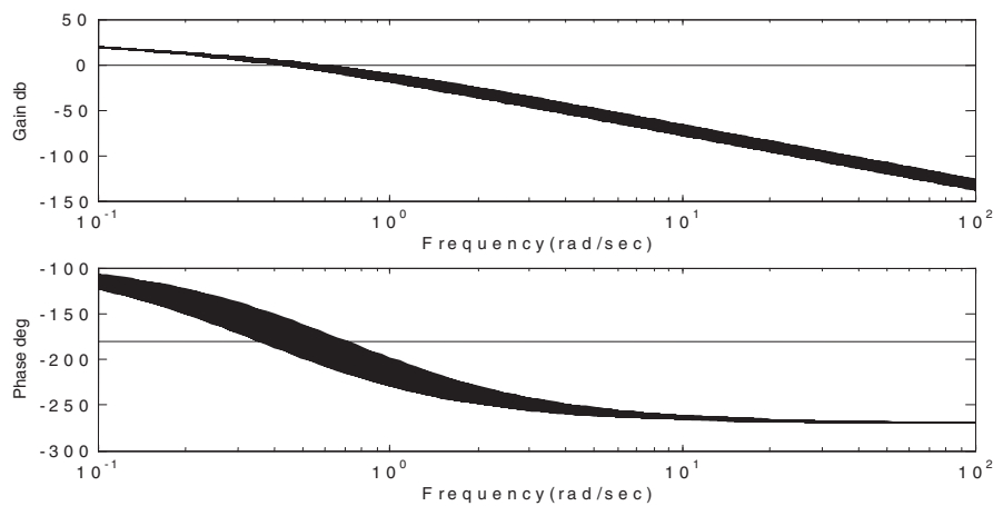
Figure 9.9 Stability from the Bounds of the Bode plots.
