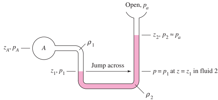
Fig. 2.9 Simple open manometer for measuring p_A relative to atmospheric pressure.
