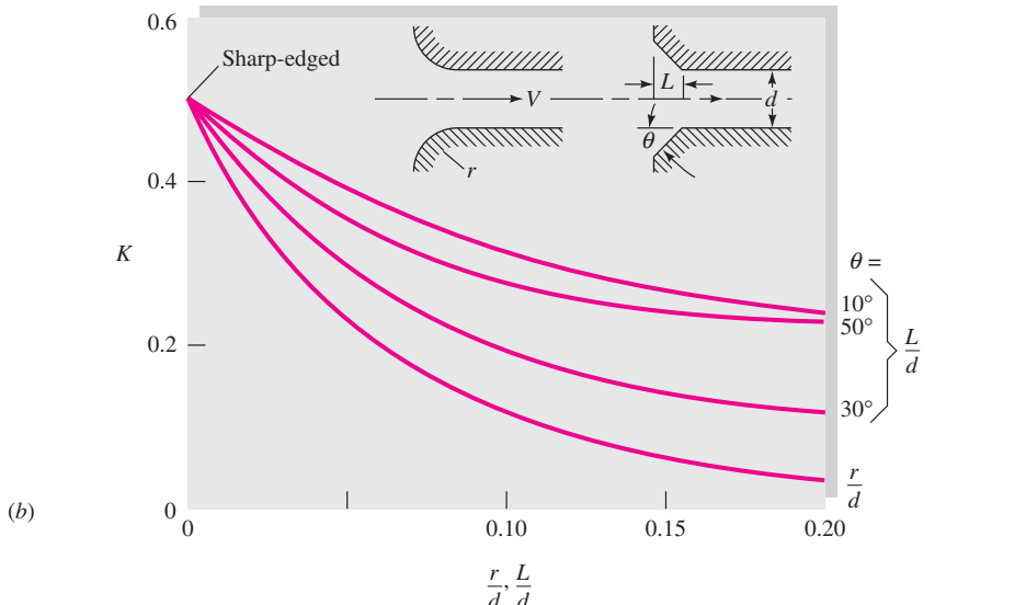
Fig. 6.21 Entrance and exit loss coefficients: (a) reentrant inlets; (b) rounded and beveled inlets. Exit losses are K \approx 1.0 for all shapes of exit (reentrant, sharp, beveled, or rounded). (From Ref. 37.)
