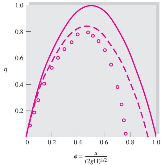
Fig. 11.27 Efficiency of an impulse turbine calculated from Eq. (11.41): solid curve = ideal, \beta = 180^\circ , C_v = 1.0 ; dashed curve = actual, \beta = 160^\circ , C_v = 0.94 ; open circles = data, Pelton wheel, diameter = 2 ft.
