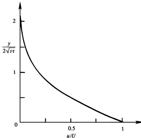
FIGURE 8.13 Similarity solution of laminar flow due to an impulsively started flat plate. Using these scaled coordinates, all flow profiles like those shown on Figure 8.12 will collapse to the same curve. The factor of two in the scaling of the vertical axis follows from (8.30).
