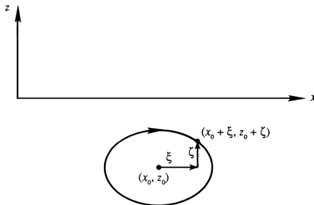
FIGURE 7.3 Orbit of a fluid particle below a linear surface wave. The average position of the particle is (x_0, z_0) , and \xi(t) and \zeta(t) are small time-dependent displacements in the horizontal and vertical directions, respectively. When the surface wave is sinusoidal, travels to the right, and has small amplitude, the fluid particles below the surface traverse closed elliptical orbits in the clockwise direction.
