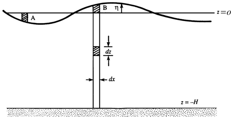
FIGURE 7.6 Calculation of potential energy of a fluid column. Here work must be done to push the liquid surface down below z = 0 (A), and lift the liquid surface up above z = 0 (B).
