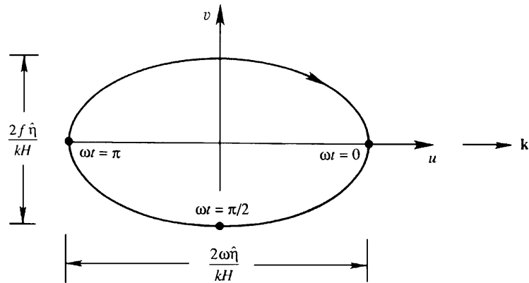
FIGURE 13.15 Particle orbit in a gravity wave traveling in the positive x -direction. Looking down on the surface, the orbit is an ellipse having major and minor axes proportional to the wave frequency \omega and the inertial frequency f . Velocity components corresponding to \omega t = 0, \pi/2 , and \pi are indicated.
