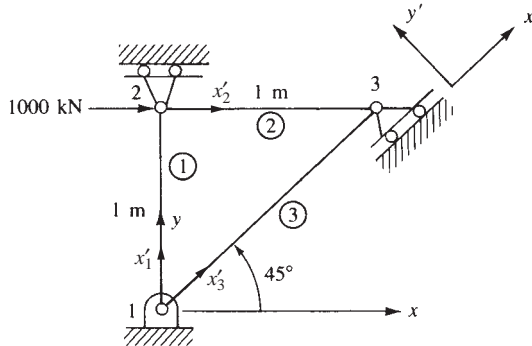
Figure 3–24 Plane truss with inclined support
