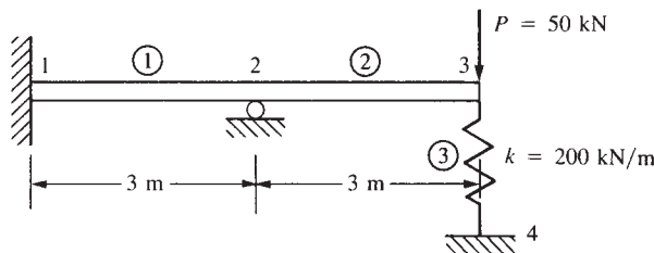
Figure 4–14 Beam example
