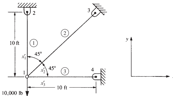
Figure 3–15 Plane truss
