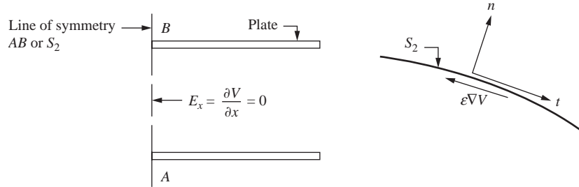
Figure 14–28 Neumann-type derivative boundary conditions on electric field intensity (Line AB is a geometric and potential symmetry line)
