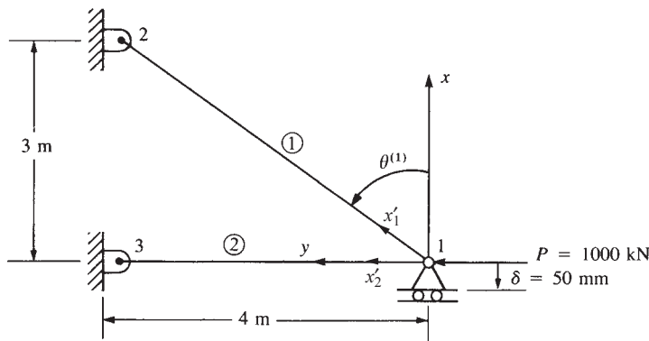
Figure 3–16 Two-bar truss
