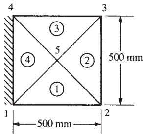
Figure 15–11 Discretized plate subjected to a temperature change
