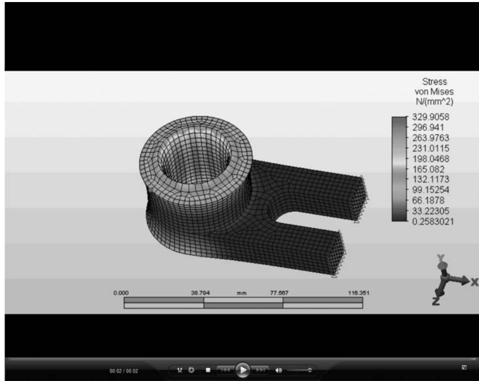
Figure 15–13 von Mises stress plot for a solid part subjected to 100^{\circ}\text{C} temperature rise inside the surface of the hole (See the full-color insert for a color version of this figure.)
