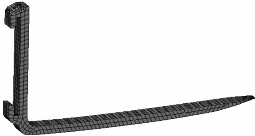
Figure P11–20 Fork from forklift showing dimensions (all dimensions in mm) and typical finite element model (Compliments of Jay Emmerich)
