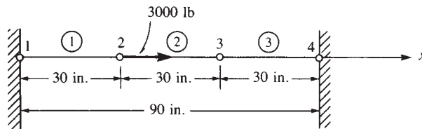
Figure 3–4 Three-bar assemblage
