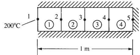
Figure 13–15 Discretized model of Figure 13–14
