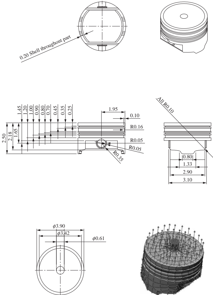
Figure P11–26 Piston head subjected to pressure load (dimensions in inches) and typical finite element model (Compliments of Robert Jablonsky)
