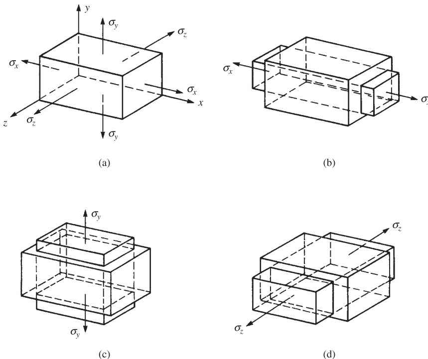
Figure C-4 Element subjected to normal stress acting in three mutually perpendicular directions
