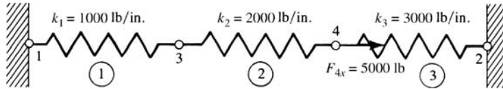
Figure 2–24 Spring assemblage
