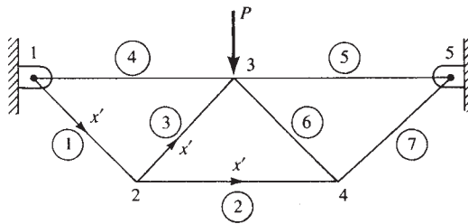
Figure B–7 Truss for wavefront solution
