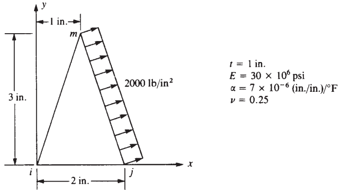
Figure 15–10 Plane stress element subjected to mechanical loading and a temperature change
