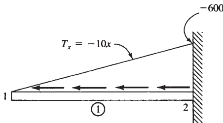
Figure 3–31 One-element model
