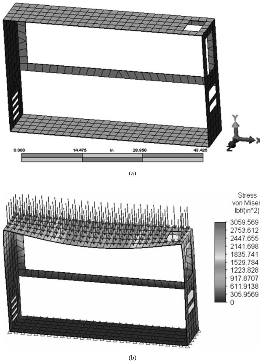
Figure 12–12 (a) Finite element model of a computer case composed of plate bending elements and (See the full-color insert for a color version of this figure.) (b) the pressure load, boundary conditions, and resulting von Mises stress (by Nicholas Dachniwskyj)
