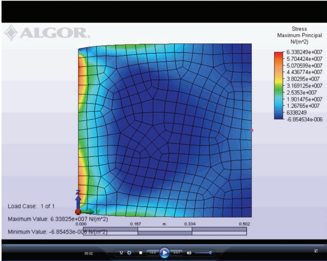
Figure 15–12 Discretized plate showing displaced plate superimposed with maximum principal stress plot in Pa.
