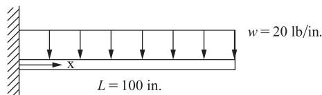
Figure 4–30 Cantilever beam subjected to uniformly distributed load
