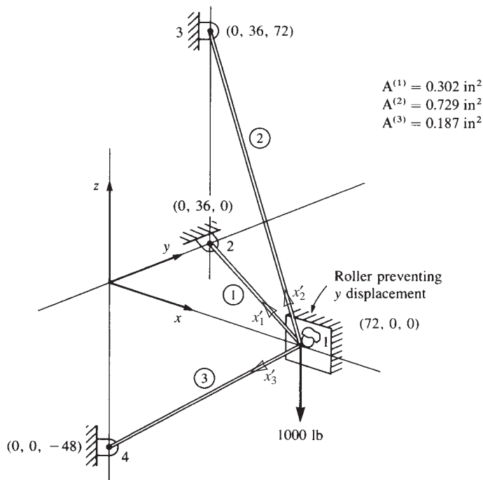
Figure 3–19 Space truss
