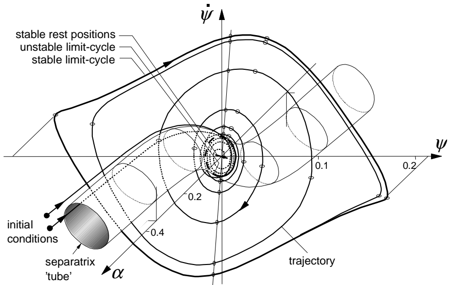
Fig. 6.27. Solutions in the three-dimensional state space. System with non-linear tyre and dry friction ( \underline{V} = 6.66 , \underline{\sigma} = 3 , \underline{e} = 0 , \underline{k}^* = \underline{k} = \underline{\delta} = 0 , \underline{K} = 0.0035 ). Line piece for possible rest positions, unstable and stable limit-cycle. Tube shaped separatrix separating space of trajectories leading to a rest position from the space of solution curves leading to the stable limit-cycle.
