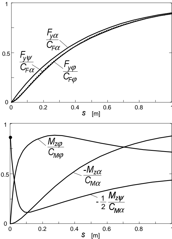
Fig. 9.15. Step response curves of the side force and of the aligning torque to side slip \alpha , turn slip (path curvature) \phi and steer angle \psi .
