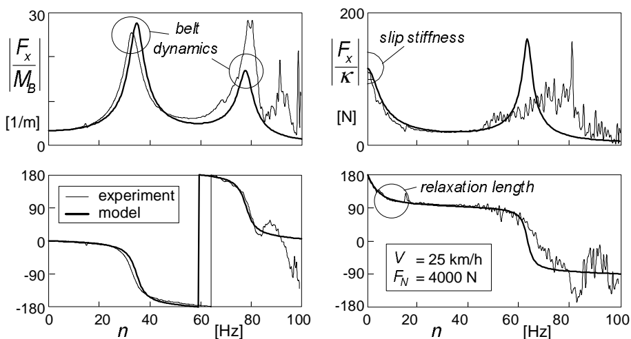
Fig. 9.41. Measured and calculated in-plane frequency response functions at an average braking force of 450N and assessed at a braking force standard deviation of 75N.
