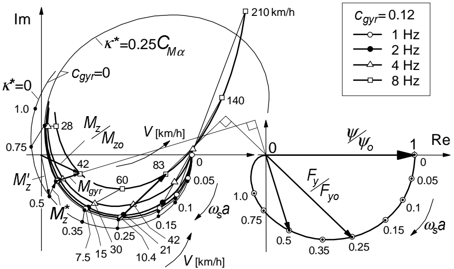
Fig 5.38. The influence of the frequency of the yaw oscillation on the dynamic response according to the simple approximate model extension using the gyroscopic couple due to the lateral tyre deflection time rate of change.
