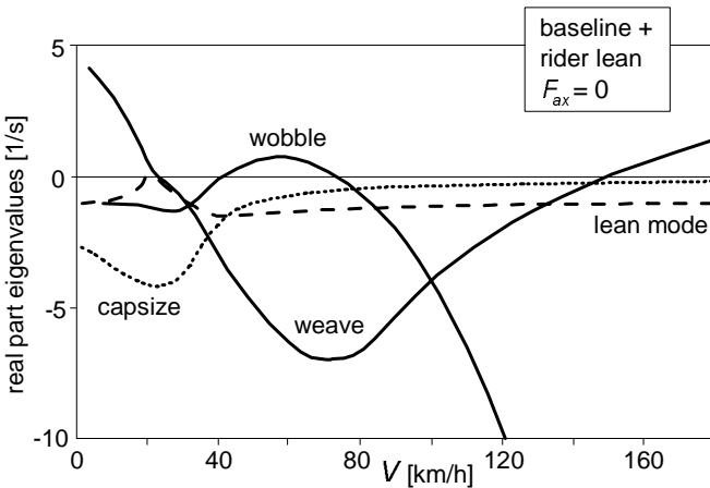
Fig. 10.11. The stability diagram with the rider lean degree of freedom introduced.
