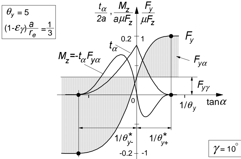
Fig. 3.27. Basic configuration of the characteristics vs side slip at camber angle \gamma=10 deg.
