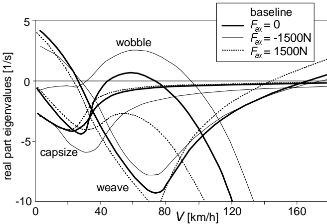
Fig. 10.10. Effect of the application of braking ( F_{ax}, F_{x1,2} < 0 ) and driving forces ( F_{ax}, F_{x2} > 0 ) on the stability diagram (baseline configuration).
