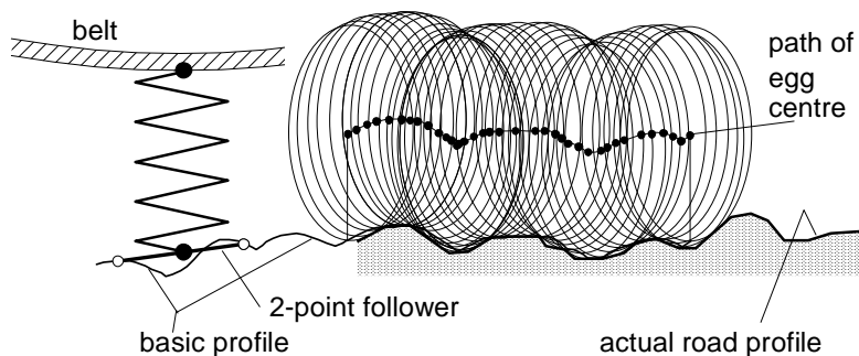
Fig. 9.57. The egg generating the basic road profile and three-point follower moving over it.
