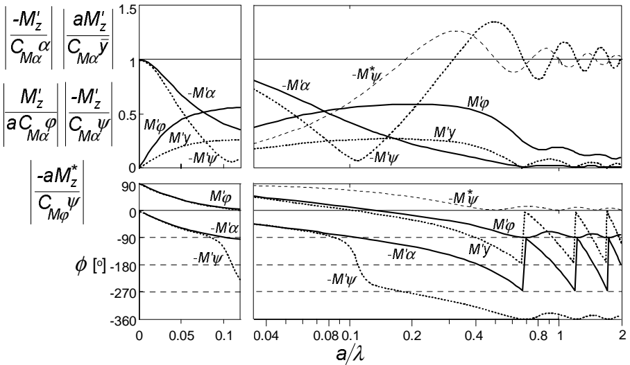
Fig. 5.34. Frequency response functions of string model with tread elements for the aligning torque with respect to various motion input variables. Same conditions as in Fig.5.33. The response functions of the moment due to tread width M'_z have been added.
