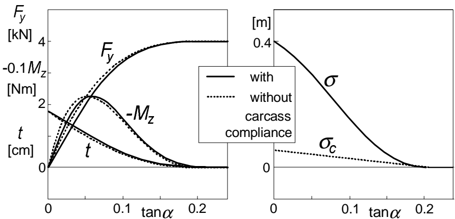
Fig. 9.7. Steady-state side slip force and moment characteristics and the relaxation length of the brush model (the contact patch) and of the model including the flexible carcass through which the brush model is attached to the wheel plane.
