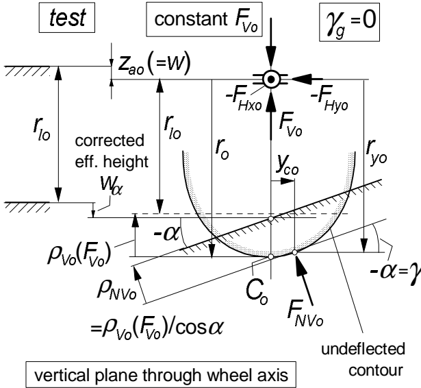
Fig. 9.72. Suggested test configuration performed at constant vertical wheel load F_{V_o} to assess effective road plane height and slopes (on frictionless surface). The for transverse slope corrected effective height w_\alpha
