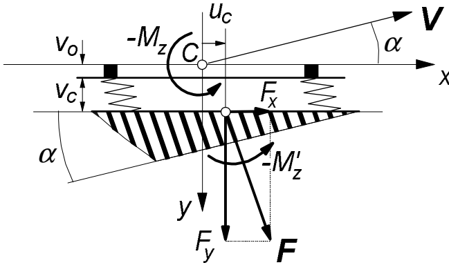
Fig. 3.19. Extended tyre brush model showing off set and deflection of carcass line (straight and parallel to wheel plane).
