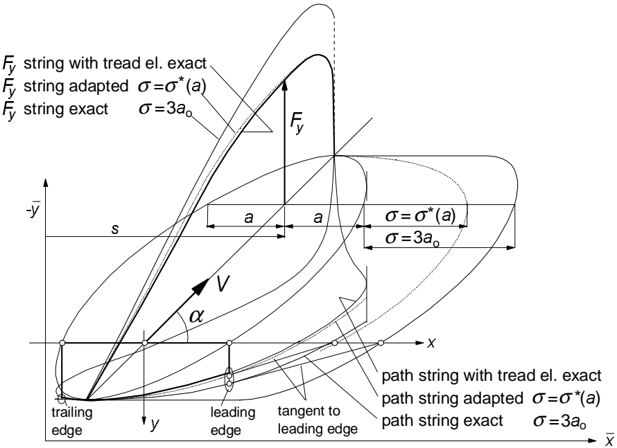
Fig. 5.49. Paths of contact points and variations of the side force according to three models.
