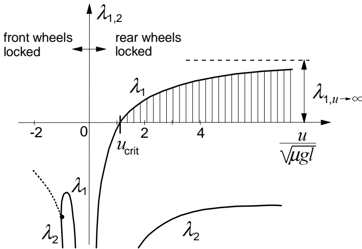
Fig. 3.42. Real (part of the) eigenvalues of the substitutive linear system with constant coefficients.
