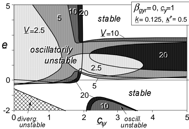
Fig. 6.12. Same as Fig.6.11 but with some damping. Areas of instability at different levels of speed.
