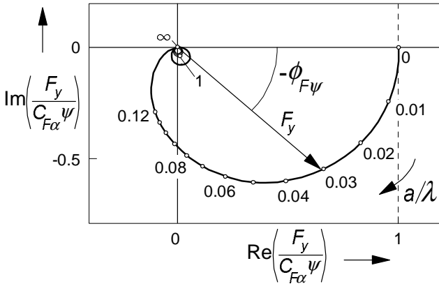
Fig.5.17. Nyquist plot of the non-dimensional frequency response function of the side force F_y with respect to the wheel yaw angle \psi . Parameter: \sigma = 3\alpha .
