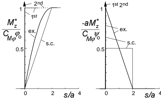
Fig. 5.22. Step response of the moment due to tread width to turn slip (path curvature) and yaw angle for exact and approximations: ex.: exact (brush model); s.c.: straight connection (linear interpolation); 2nd: second-order approximation; 1st: first-order approximation.
