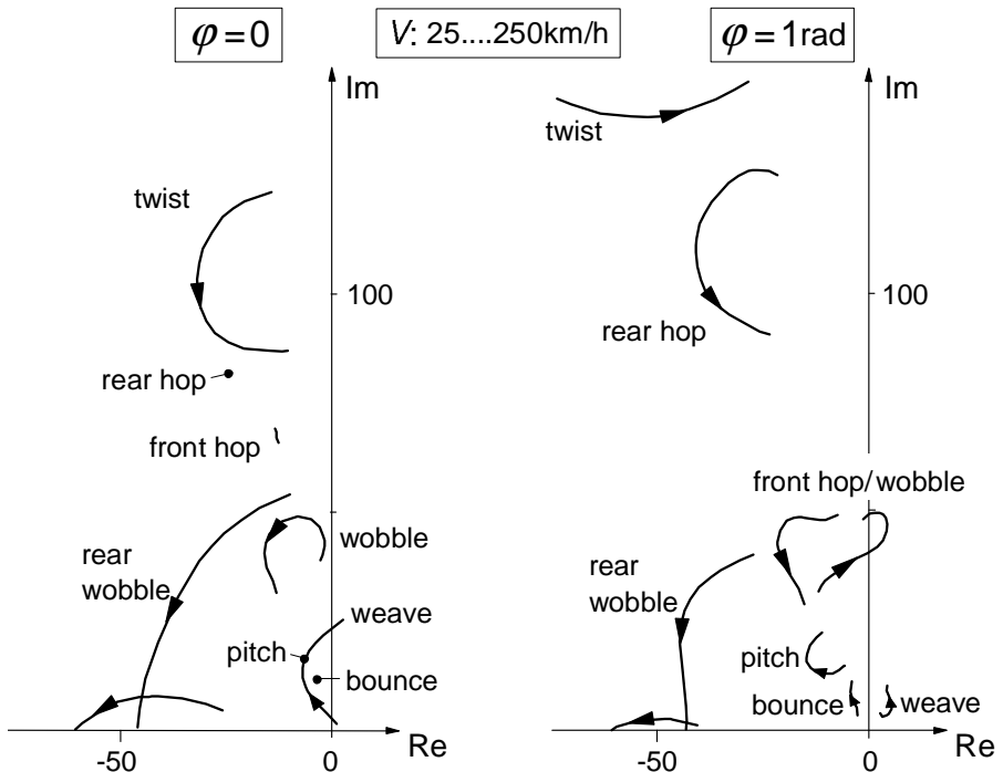
Fig. 10.29. Eigenvalues of Koenen's motorcycle model at straight ahead running ( \phi = 0 ) and at a roll angle of one radian. The speed varies from 25 to 250 km/h.
