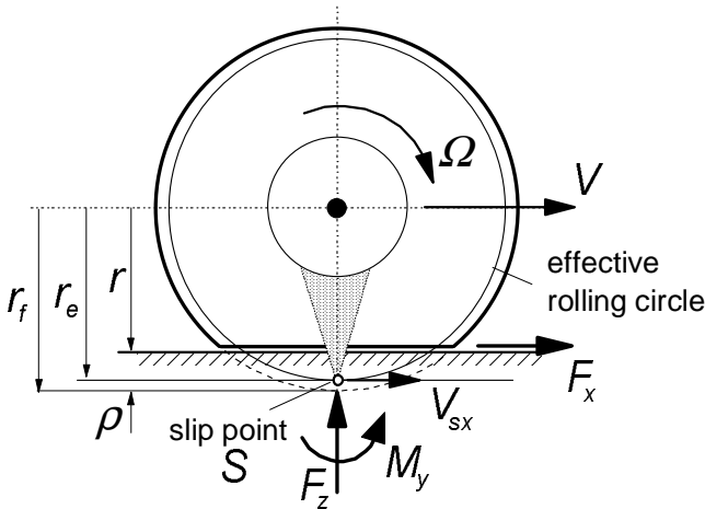
Fig. 8.11. The rolling wheel subjected to longitudinal slip (slip speed V_{sx} )
