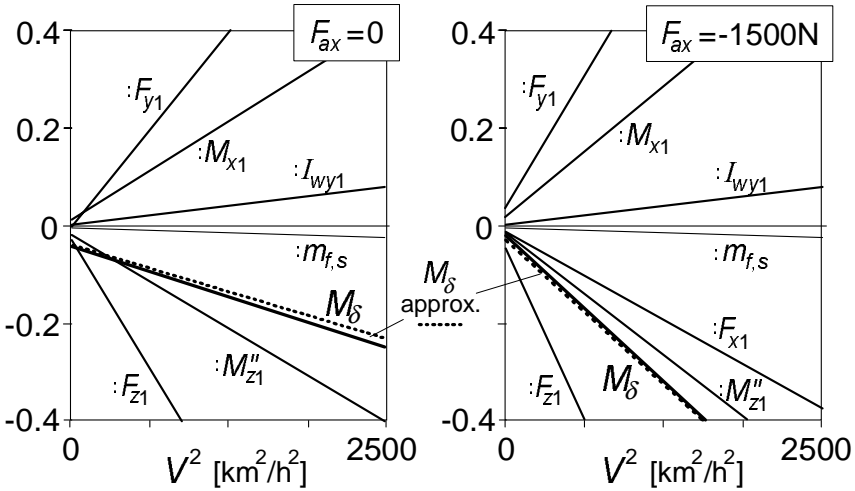
Fig. 10.20. The non-dimensional steer torque ( M_\delta/(F_{z10}l) ) and its components (cf. Eq.(10.147)) per unit non-dimensional path curvature l/R . In M''_{z1} the F_{x1} contribution is omitted.
