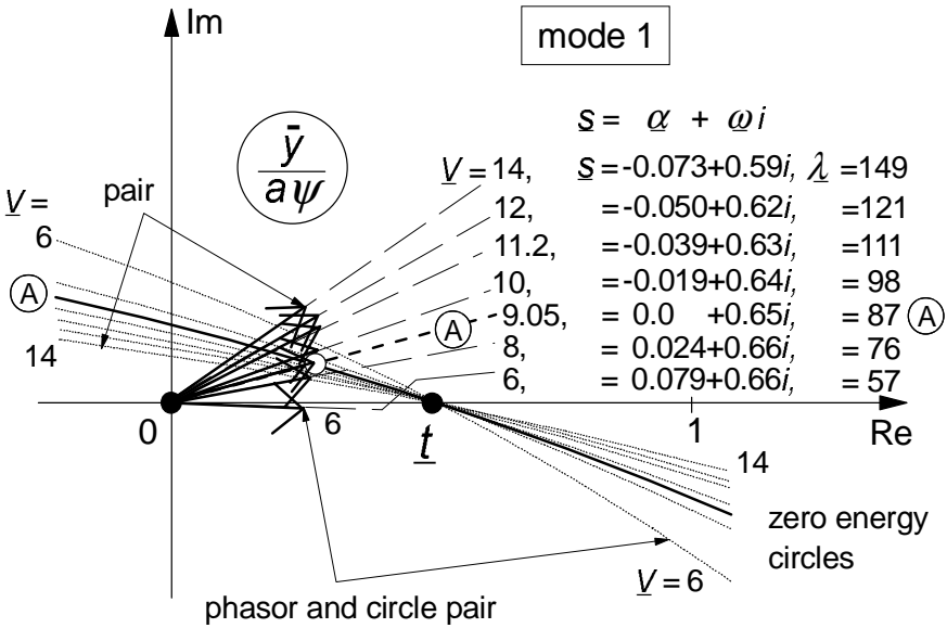
Fig. 6.22. System of Fig.6.8 with gyroscopic coupling making stability speed dependent. Circle segments and phasors of mode shapes of mode 1 for a series of speed values covering the range in which points A and B of Fig.6.8 are located. At increasing speed the phasor crosses the circle at \underline{V} = 9.05 into the stable domain.
