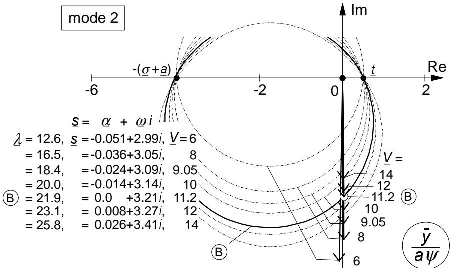
Fig. 6.23. Circles and phasors of mode shapes of mode 2 for same series of speed values as in Fig.6.22. At increasing speed the phasor crosses the circle at \underline{V} = 11.2 towards its inside which means: entering the unstable domain.
