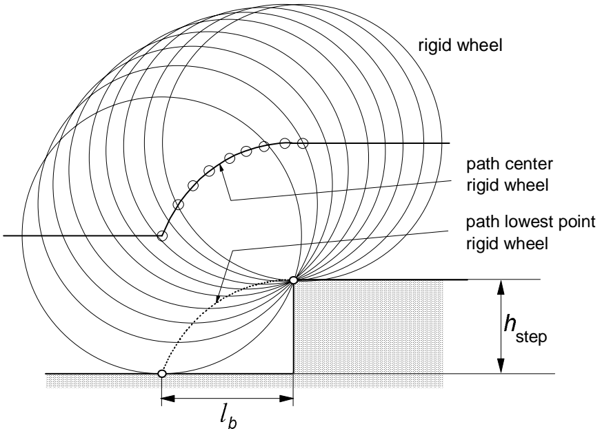
Fig. 9.53. The rigid wheel rolling over an upward step change in road level.
