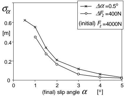
Fig. 7.10. Relaxation lengths resulting from small step changes in slip angle or wheel load, as function of slip angle level, Higuchi (1997).
