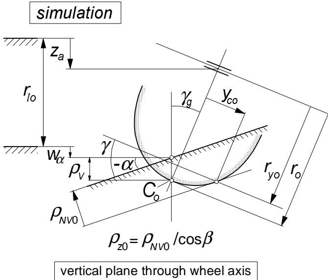
Fig. 9.73. The use of the (corrected) effective road inputs, which are calculated as function of the horizontal position of point C_o , in a simulation where a global wheel camber angle \gamma_g may occur.
