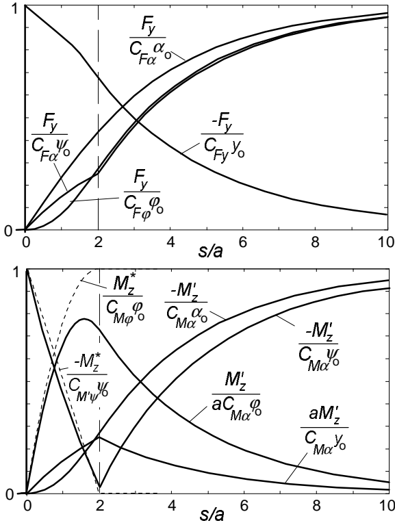
Fig. 5.10. Step response of side force F_y , aligning torque M_z' and tread width moment M_z^* to side slip \alpha , lateral displacement \tilde{y} , turn slip \phi and yaw angle \psi . Computed for string model with deflection relaxation length \sigma = 3a .
