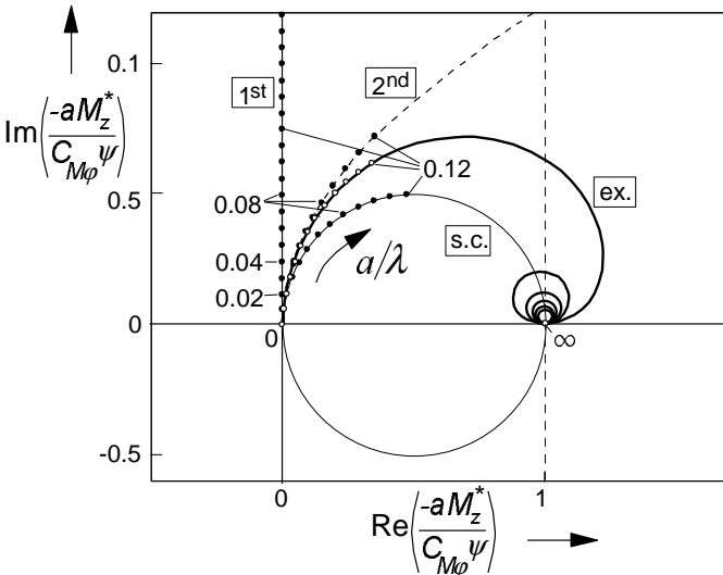
Fig.5.26. Nyquist plot of the frequency response function of the torque due to tread width -M_z^* with respect to the wheel yaw angle \psi . ex.: exact (brush); s.c.: straight connection (linear interpolation); 2nd: second-order app.; 1st: first-order approx.
