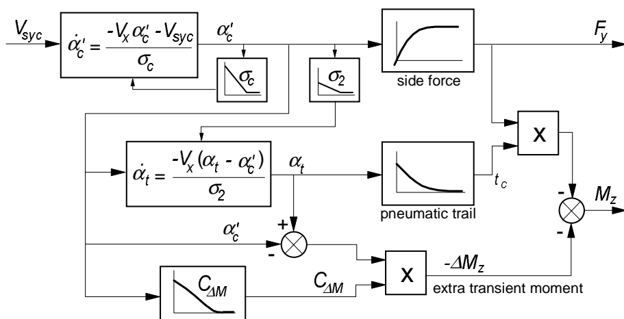
Fig. 9.9. Block diagram of the non-linear model of the contact patch (tread) also valid for larger slip angle variations.
