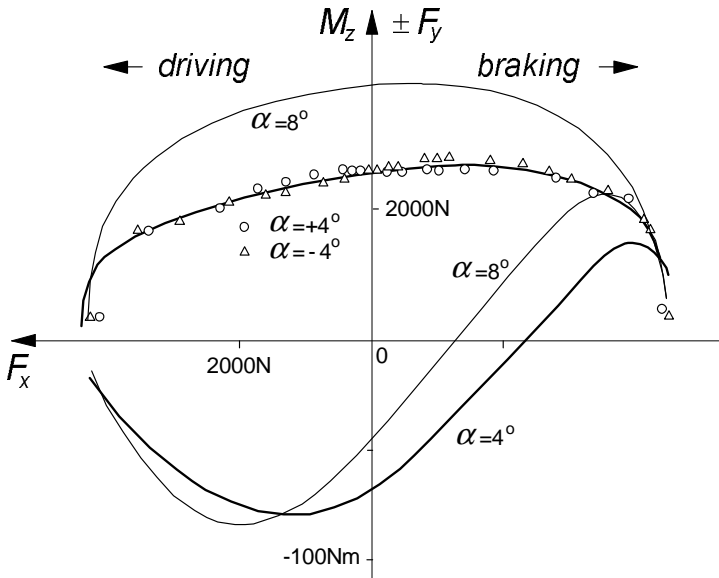
Fig. 3.18. Combined slip side force and moment versus longitudinal force characteristics measured at two values of the slip angle for a 7.60-15 tyre on a dry flat surface (from Nordeen and Cortese (1963)).
