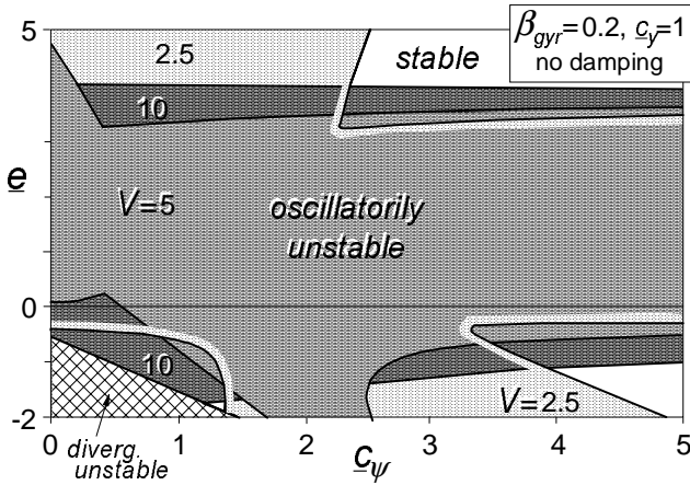
Fig. 6.14. Diagram for the case of Fig.6.11 but with gyrosopic coupling. Areas of instability at different levels of speed.
