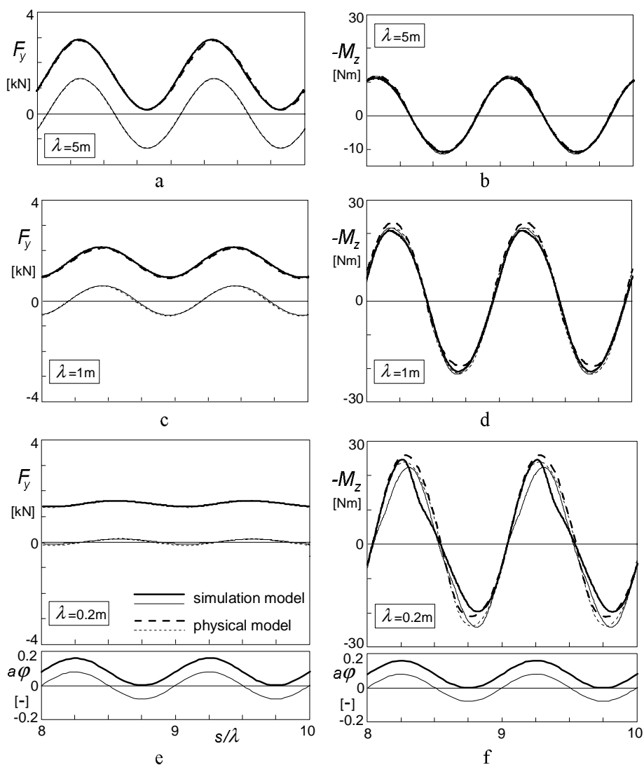
Fig.9.11. Side force and aligning torque responses of the non-linear brush simulation model with flexible carcass to sinusoidal path curvature variations (turn slip at \alpha = 0 ) of the wheel plane with an amplitude of a\varphi of 0.08 and average levels of 0 (thin curves) and 0.08 (fat curves), compared with results of the physical model (broken curves).
