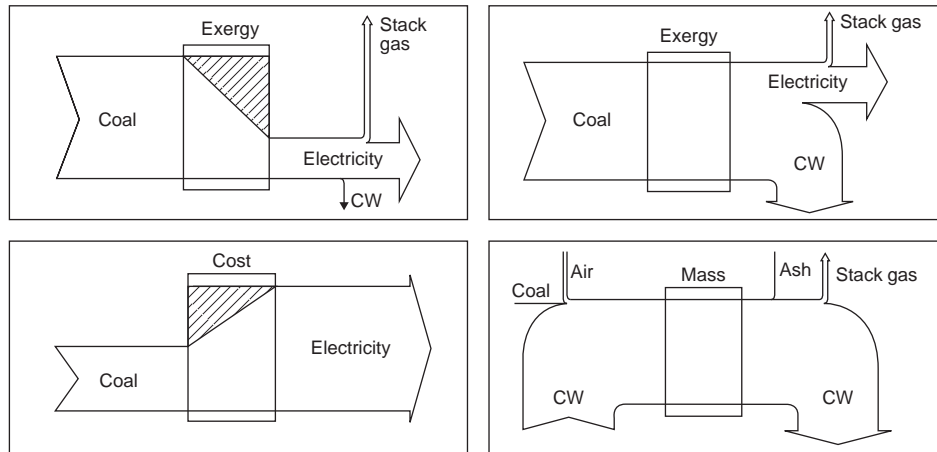
Fig. 17.9. Summary of the results of an EXCEM analysis of a coal-fired electrical generating station. Overall balances of flow rates of exergy, cost, energy and mass are shown. The rectangle in the center of each diagram represents the station. Widths of arrows are proportional to the relative magnitudes of the represented quantities. Rates of exergy consumption and cost creation are denoted by the shaded regions in the appropriate diagrams. CW denotes cooling water.
