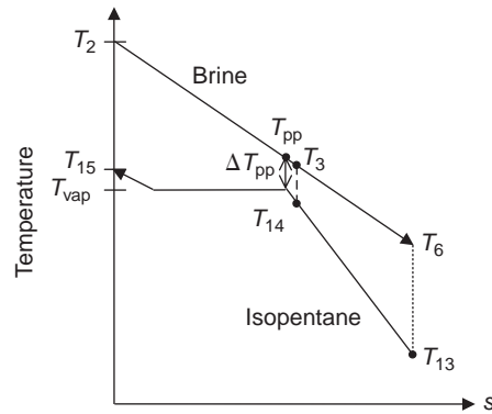
Fig. 10.44. Heat exchange process between the geothermal brine and the isopentane working fluid in Level II.
