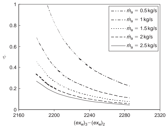
Fig. 8.5. Variation of process exergy efficiency with specific exergy difference of products for different mass flow rates of air.
