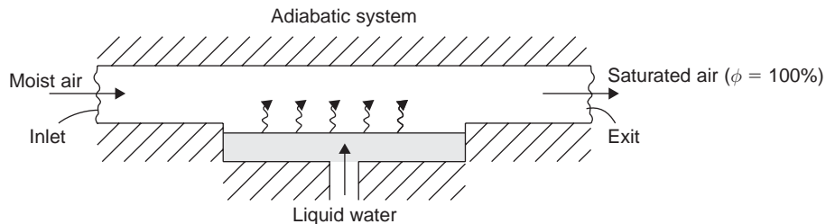
Fig. 6.3. An adiabatic saturation process.
