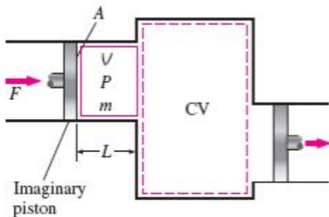
FIGURE 5-11 Schematic for flow work.
