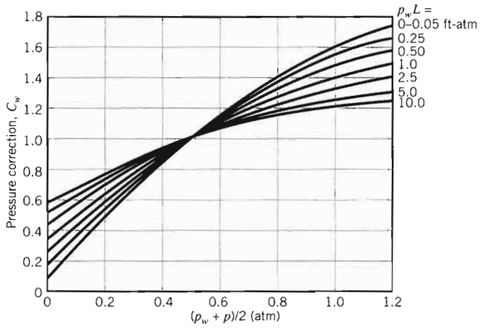
FIGURE 13.16 Correction factor for obtaining water vapor emissivities at pressures other than 1 atm ( \epsilon_{w,p \neq 1 \text{ atm}} = C_w \epsilon_{w,p = 1 \text{ atm}} ) [13]. Used with permission.
