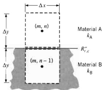
FIGURE 4.7 Conduction between adjoining, dissimilar materials with an interface contact resistance.
