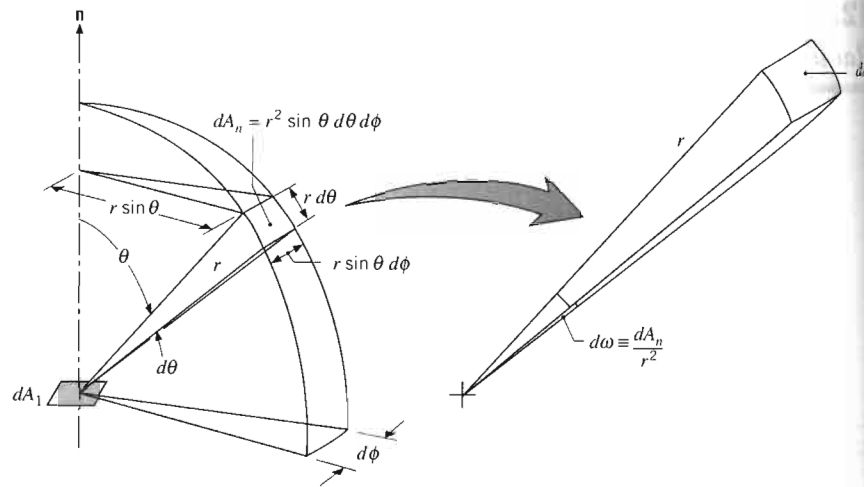
FIGURE 12.6 The solid angle subtended by dA_n at a point on dA_1 in the spherical coordinate system.
