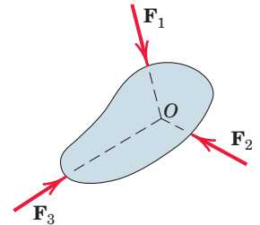
(a) Three-force member
