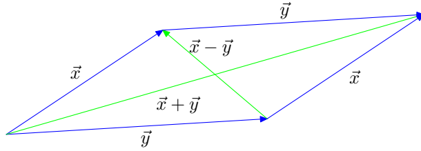
FIGURE 3. To the parallelogram identity.
