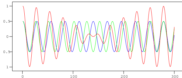
FIGURE 12. Two oscillation with unharmonious frequencies and the appearing dissonance. Click to listen the blue and green pure harmonics and red dissonance .
