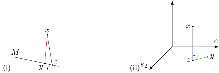
FIGURE 6. (i) A smaller distance for a non-perpendicular direction; and (ii) Best approximation from a subspace
