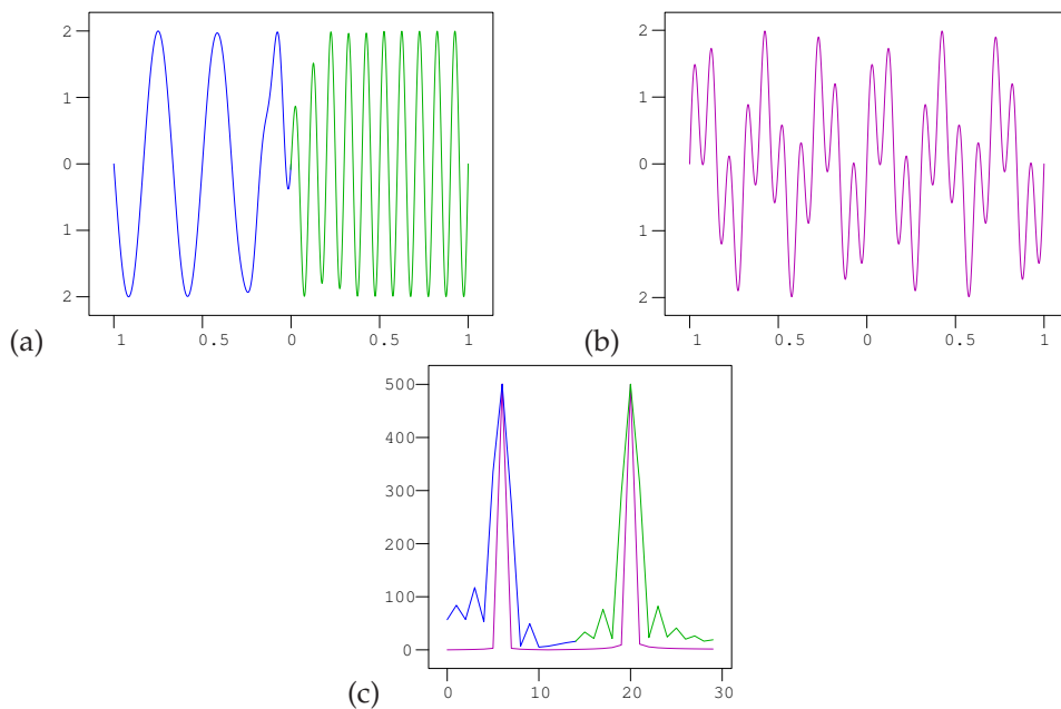
FIGURE 15. Limits of the Fourier analysis: different frequencies separated in time
