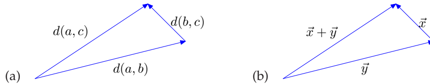
FIGURE 1. Triangle inequality in metric (a) and normed (b) spaces.
