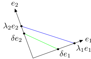
FIGURE 16. Distance between scales of orthonormal vectors
