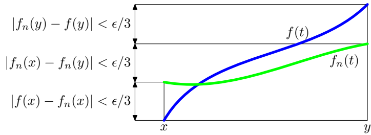
FIGURE 17. The \epsilon/3 argument to estimate |f(x) - f(y)| .
