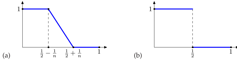
FIGURE 4. Jump function on (b) as a L_2 limit of continuous functions from (a).
