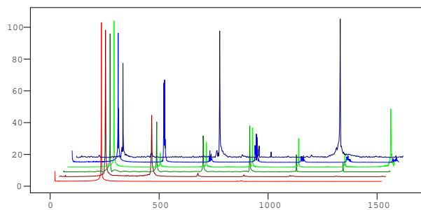
FIGURE 14. Fourier series for G5 performed on different musical instruments (same order and colour as on the previous Figure )
