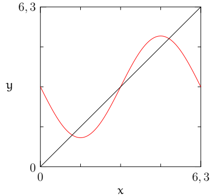
FIGURE 7. Best approximation by three trigonometric polynomials
