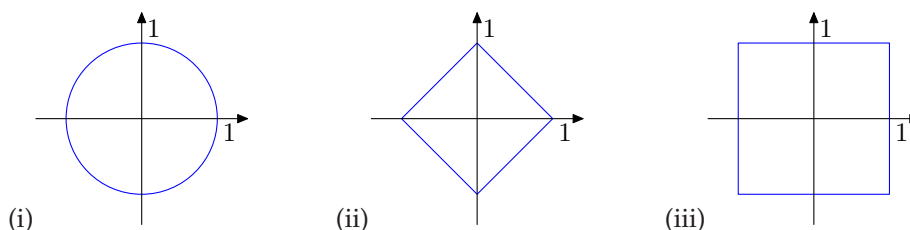
FIGURE 2. Different unit balls defining norms in \mathbb{R}^2 from Example 2.9.
