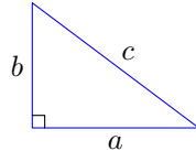
FIGURE 5. The Pythagoras' theorem c^2 = a^2 + b^2
