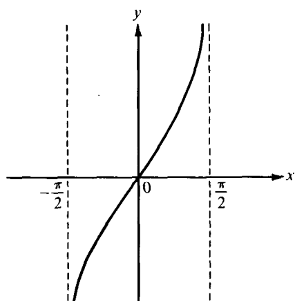
FIGURE 6.13 y = \tan x .
