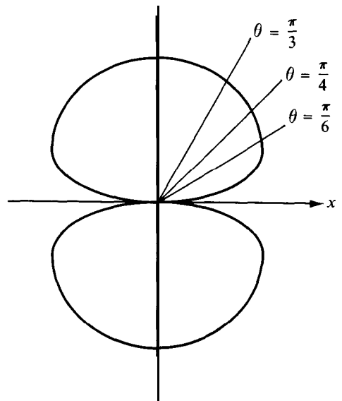
FIGURE 2.12 A figure-eight curve with polar equation r = \sqrt{|\sin \theta|} .
