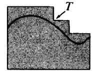
FIGURE 1.15 An ordinate set enclosed by two step regions.
