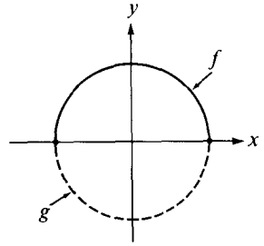
FIGURE 1.13 Graphs of two functions: f(x) = \sqrt{r^2 - x^2} , g(x) = -\sqrt{r^2 - x^2} .
