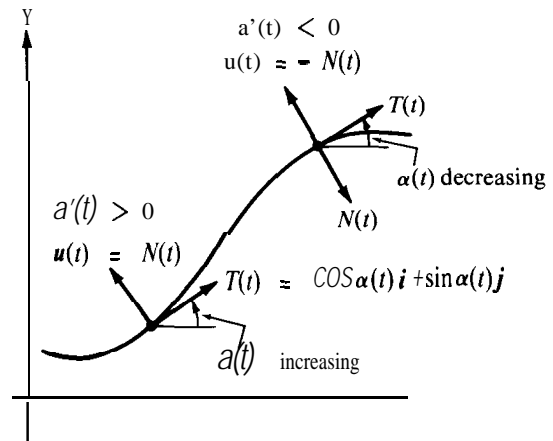
FIGURE 14.11 The angle of inclination of the tangent vector of a plane curve.
