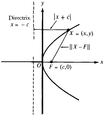
FIGURE 13.15 The parabola y^2 = 4cx .
