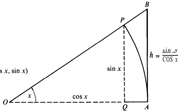
FIGURE 2.9 Geometric proof of the inequalities 0 < \cos x < \frac{\sin x}{x} < \frac{1}{\cos x} .
