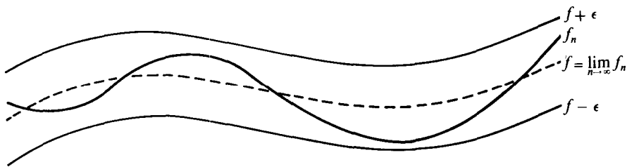
FIGURE 11.3 Geometric meaning of uniform convergence. If n \geq N , the entire graph of each f_n lies within a distance \epsilon from the graph of the limit function f .
