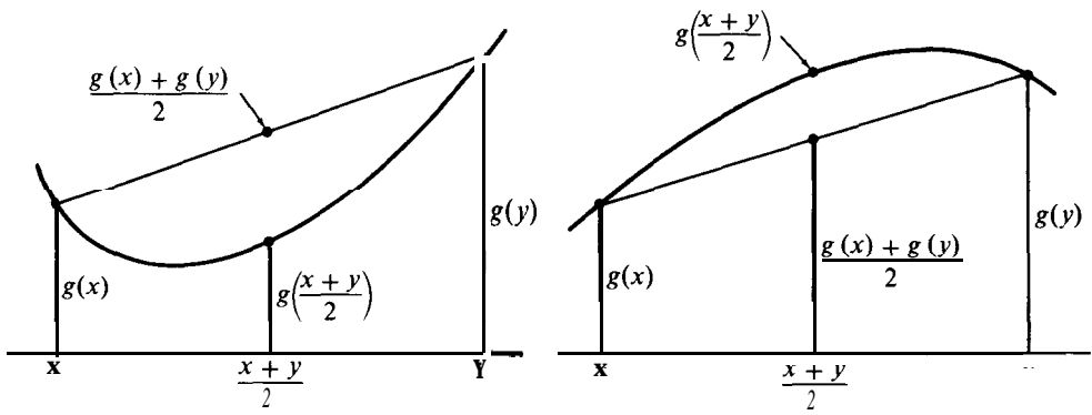
(a) A convex function
